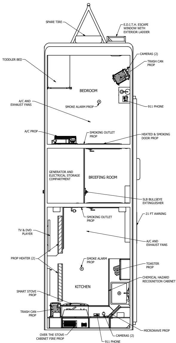
▲ 27 FT FIRE SAFETY TRAILER BEDROOM & KITCHEN
