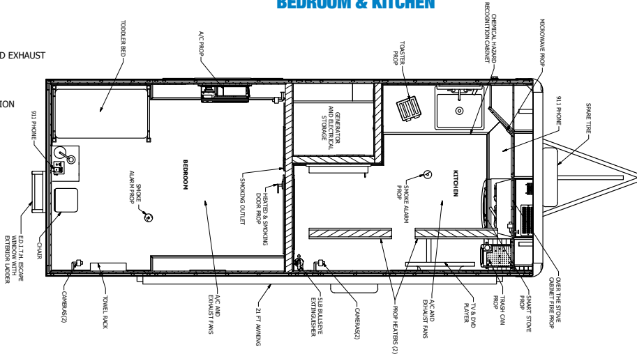
▲ 27 FT FIRE SAFETY TRAILER BEDROOM & KITCHEN
